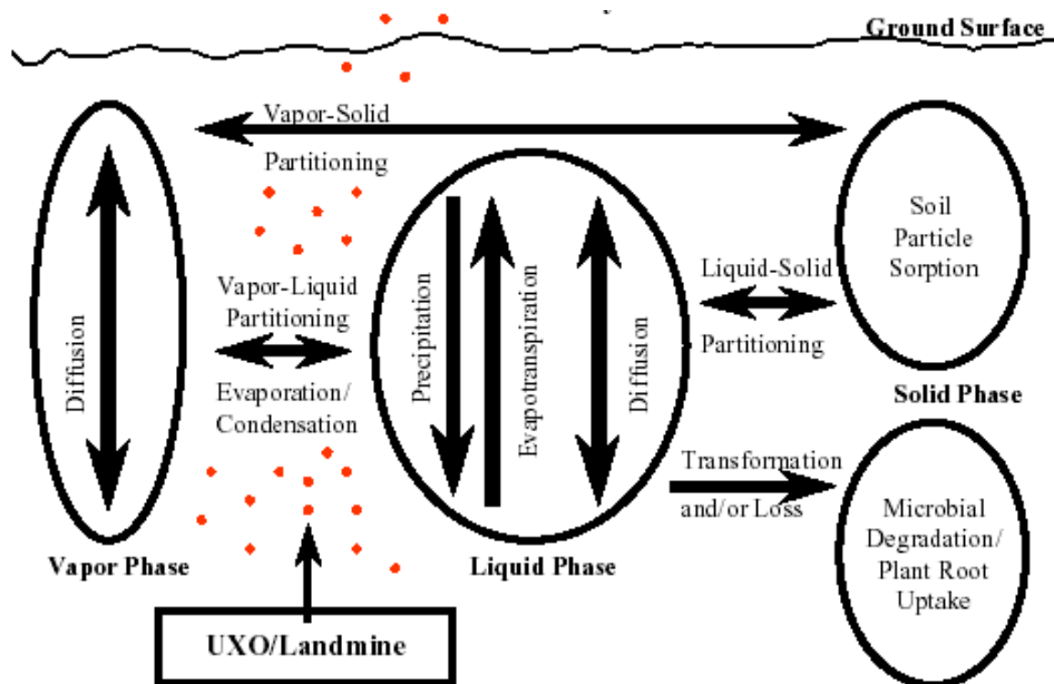
Figure 2. Chemical processes that affect TNT distributions around buried landmines or unexploded ordnance (UXO). Figure reproduced from Phelan and Barnett (2001).
