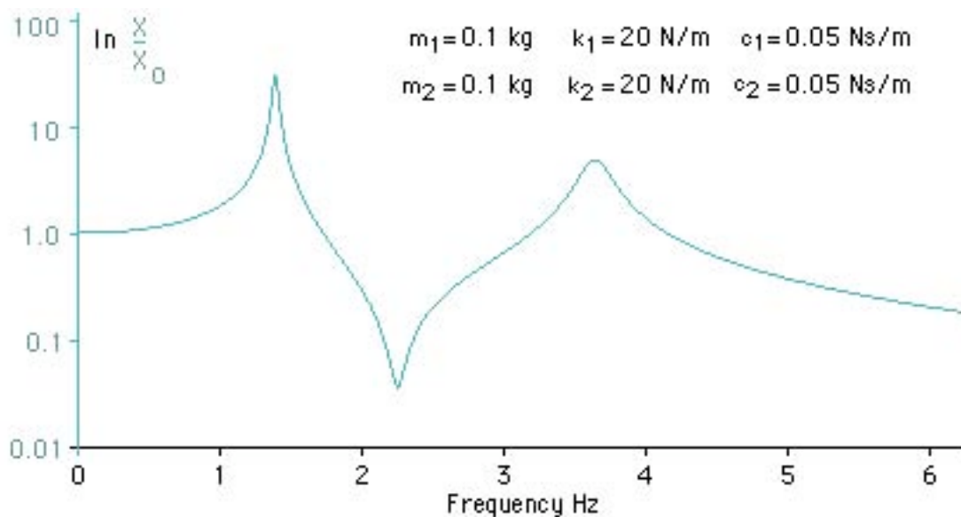
Figure 2.13 Response of damped two degree-of-freedom system
