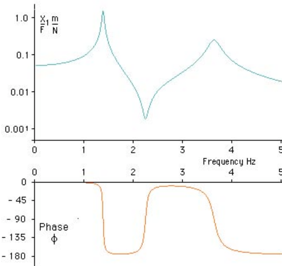
Figure 2.14 Amplitude and phase of forced response.
